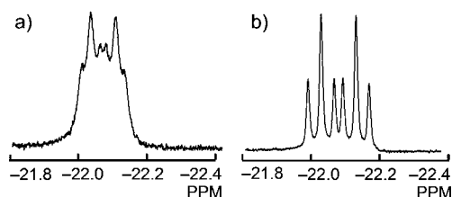
Figure 1. Hydride signals of 2 observed in a) ^1\text{H} and b) ^1\text{H}\{^{11}\text{B}\} NMR spectra.
